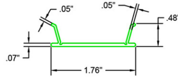
SNAP COVER
